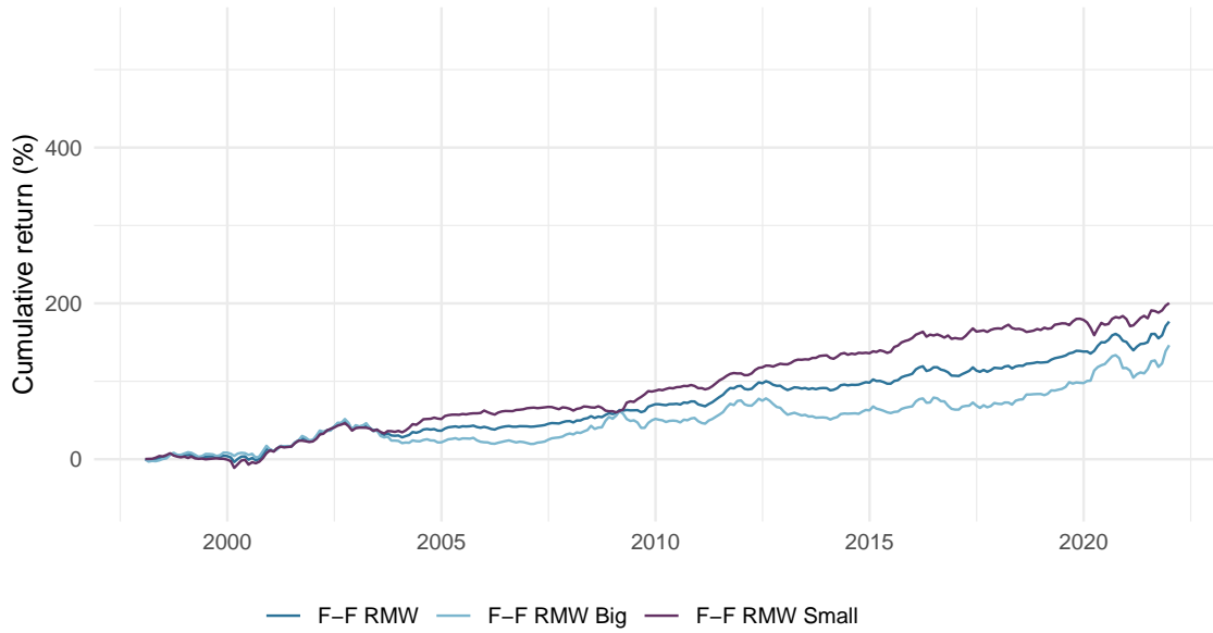
Figure 4 Cumulative returns, global RMW factor along with Big and Small versions, 1998-2021
