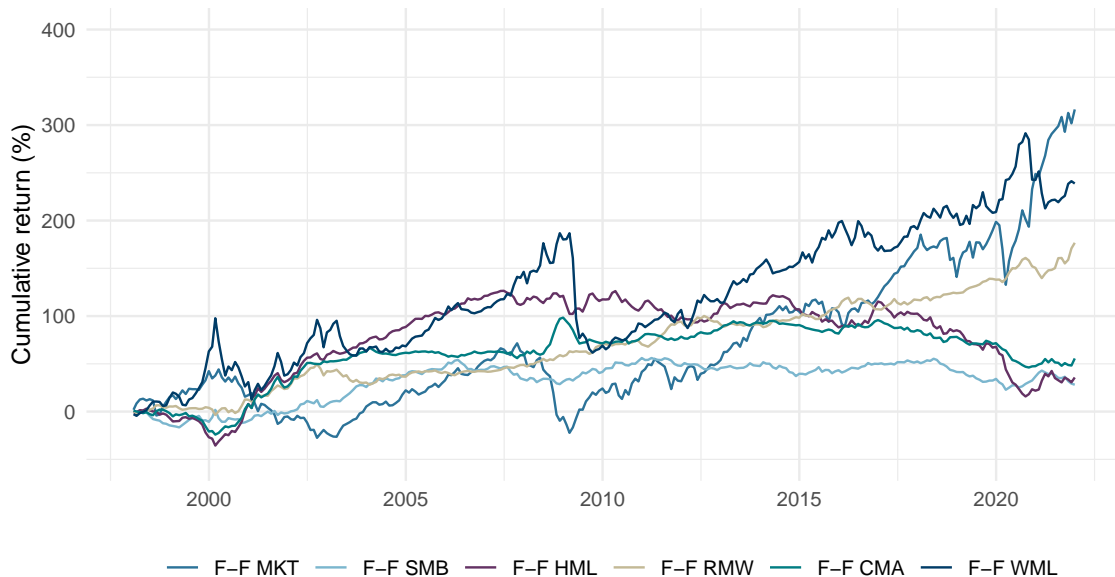
Figure 1 Cumulative returns, global Fama-French factors, 1998-2021
