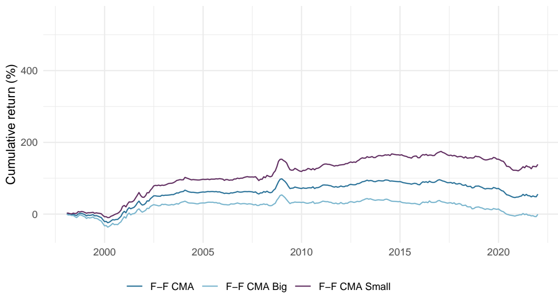
Figure 5 Cumulative returns, global CMA factor along with Big and Small versions, 1998-2021
