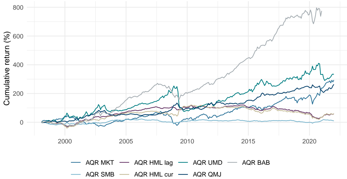
Figure 6 Cumulative returns, global AQR factors, 1998-2021
