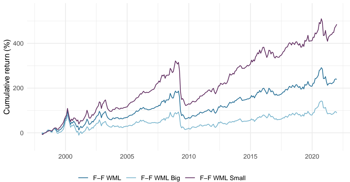
Figure 3 Cumulative returns, global WML factor along with Big and Small versions, 1998-2021
