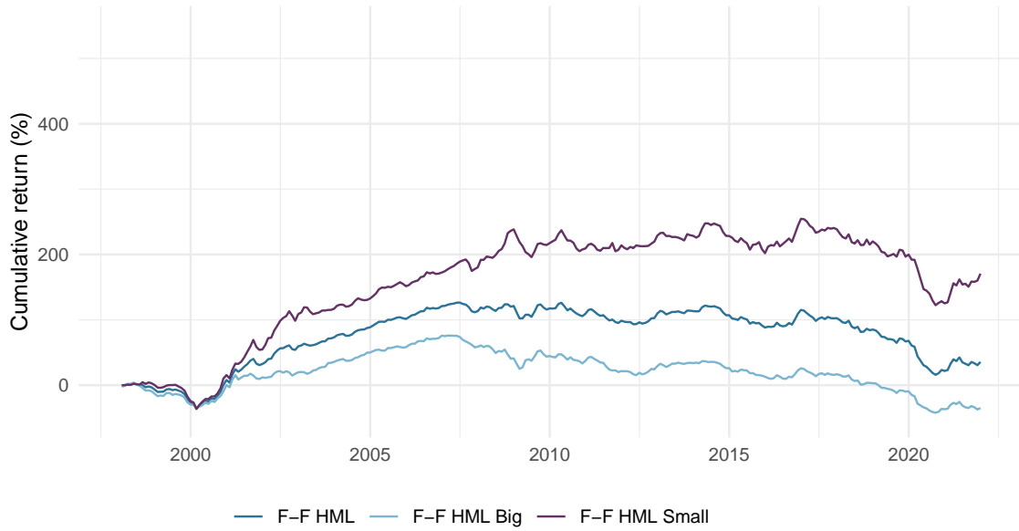
Figure 2 Cumulative returns, global HML factor along with Big and Small versions, 1998-2021
